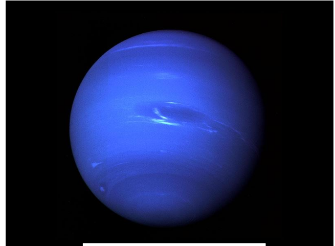
NASA/Voyager 2 image
